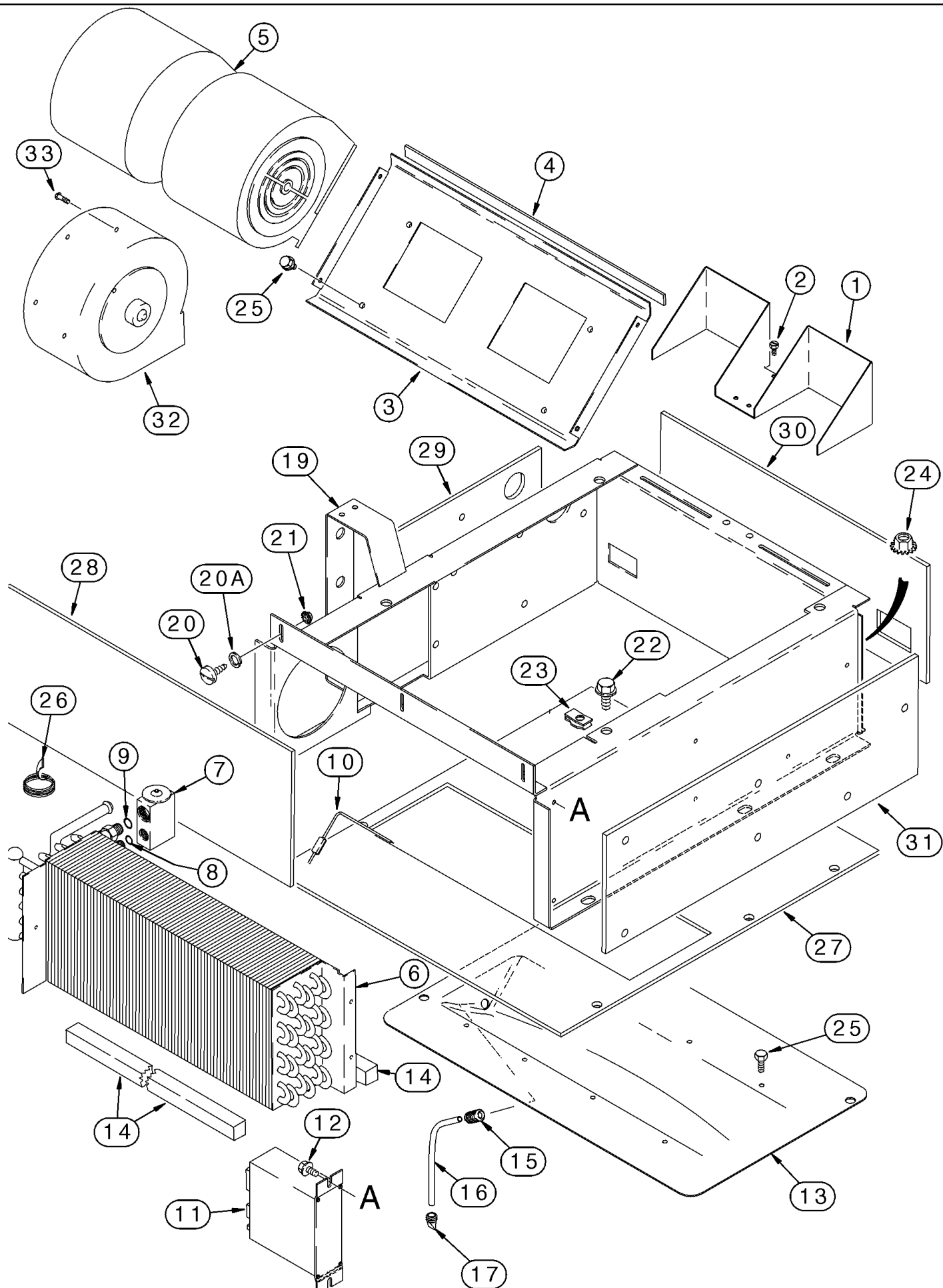
Evaporator Heater Core and Blower Mounting
